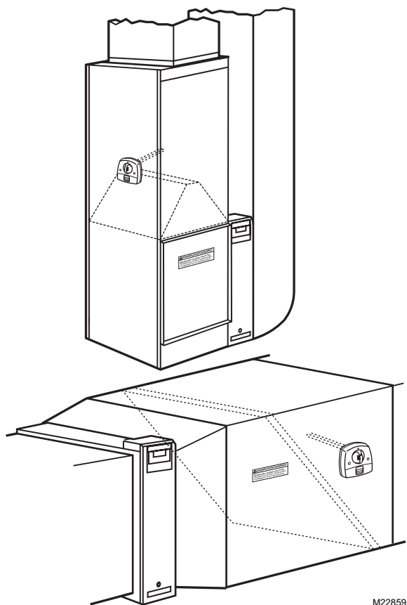
Fig. 2. Typical Surface Treatment installations.
